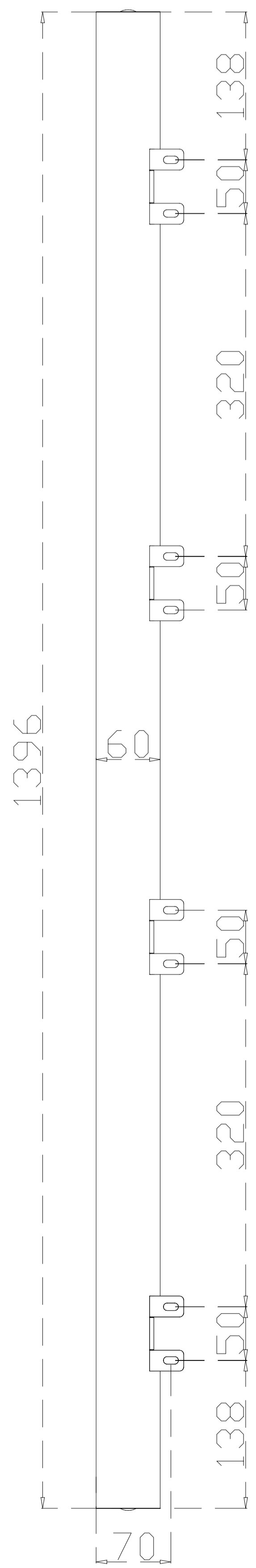
MQ 7614 * 1400 mm
